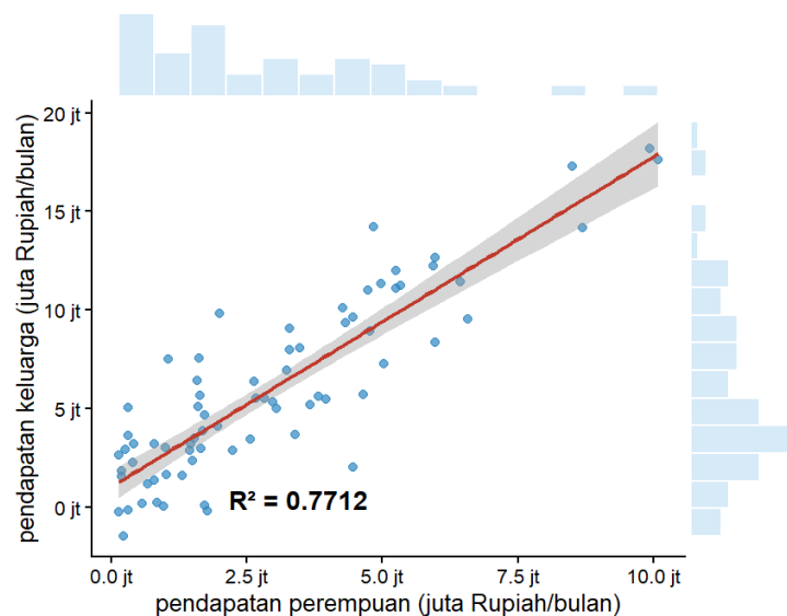
Gambar 5. Scatter plot X–Y + garis regresi
